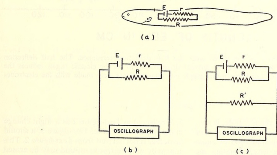
TEXT-FIG. 5. Electrical models of electric eel. a. E = electromotive force of electric organ. r = internal resistance of electric tissue. R = leakage resistance of non-electric tissue. b. Oscillograph connected to electric organ. c. Connection of a resistive load, R' , to drain current from electric organ.
