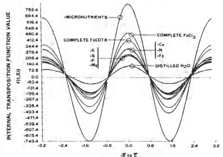
Figure 2. Multidimensional plots of plants of Juncus roemerianus grown in complete and deficient solution cultures for 68 days. The dotted, horizontal lines indicate the relative size of young plants at the beginning of the experiment. Curves shown in Figure 1 would center on the middle and fall within the upper and lower dotted lines. These dotted lines are provided to show the relative amounts of plant growth. Each curve represents the combined and relative condition of three plants in a particular series (triplicate) of deficient or complete nutrient media.
