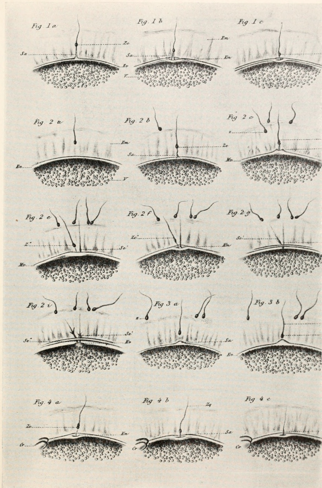
FIG. 1. Photographic reproduction of part of Plate III from Fol's paper (1879) on Asterias glacialis , the drawings of which were from the living egg. In Fig. 1, a, b, and c are three successive phases of the same zoöspERM, zc . An extension of the entrance cone is at Sa . The phase in which the zoöspERM entered is omitted here. In Fig. 2, a, b, c (d omitted) e, f, g, (h omitted) and i are seven views of the same objects; in Fig. 2, b, c, a zoöspERM, zc , is approaching. In e and f a second zoöspERM, zc' , is approaching. In g and i are extensions, Se' and Se'' , of the "cone d'exudation." Fig. 3, a, b, shows the approach of a zoöspERM to an exceptionally large cone. Fig. 4, a, b, c, shows a zoöspERM entering near region of polar bodies, Cr .
