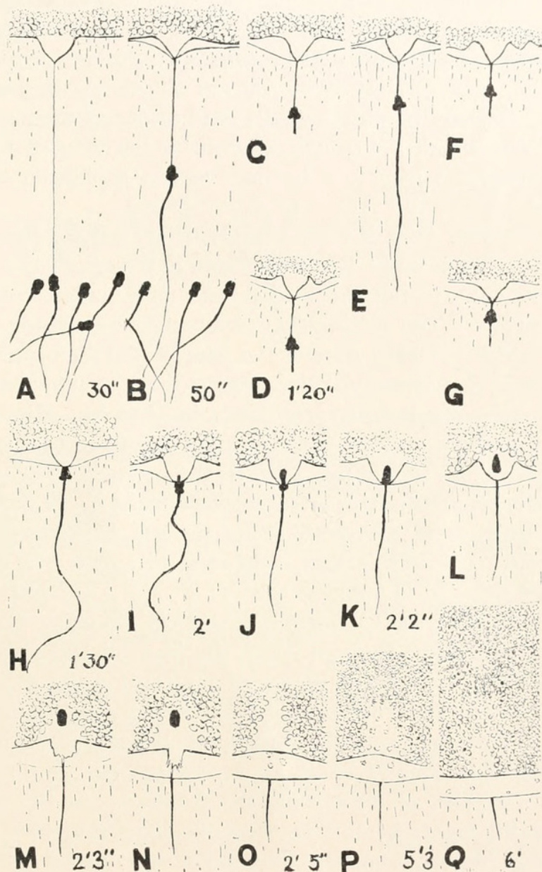
FIG. 2. Seventeen successive steps in the insemination of a starfish egg. For description see text.
