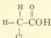
Monochloracetic acid
