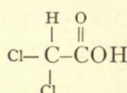
Dichloracetic acid
