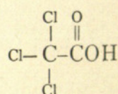
Trichloracetic acid
