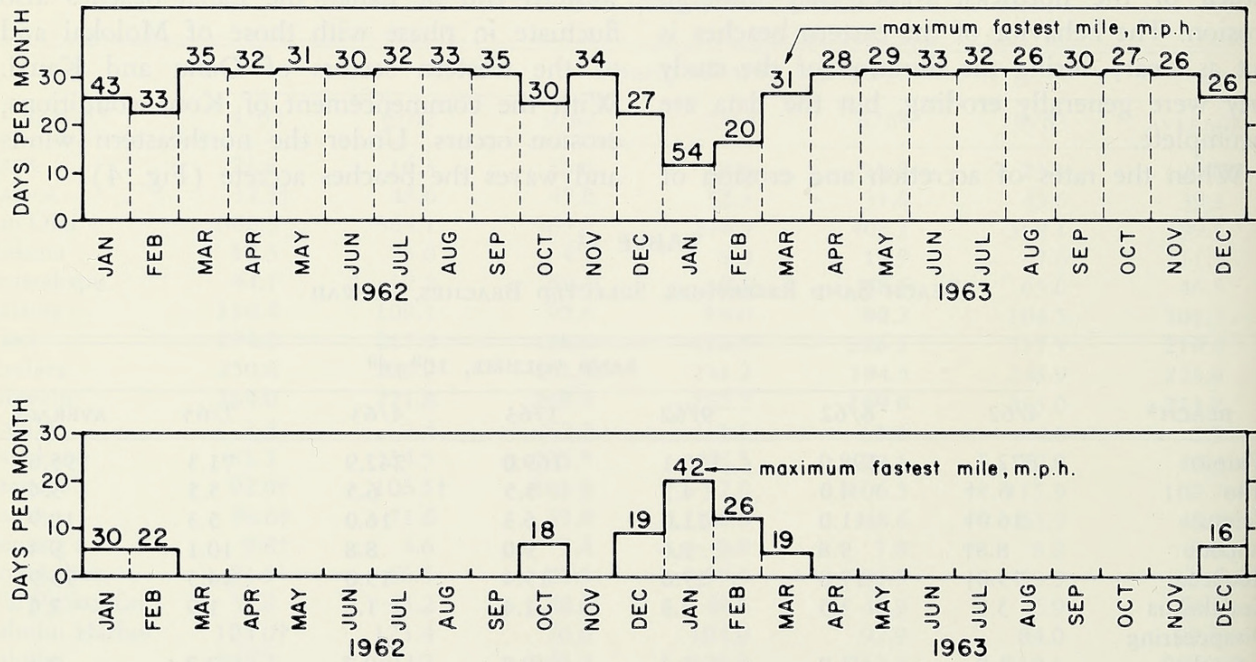
FIG. 3. Dominant winds, 1962–63. Upper, number of days per month that winds blew from the northern, eastern, and southern quadrants. Lower, number of days per month that winds blew from the southern and western quadrants.
