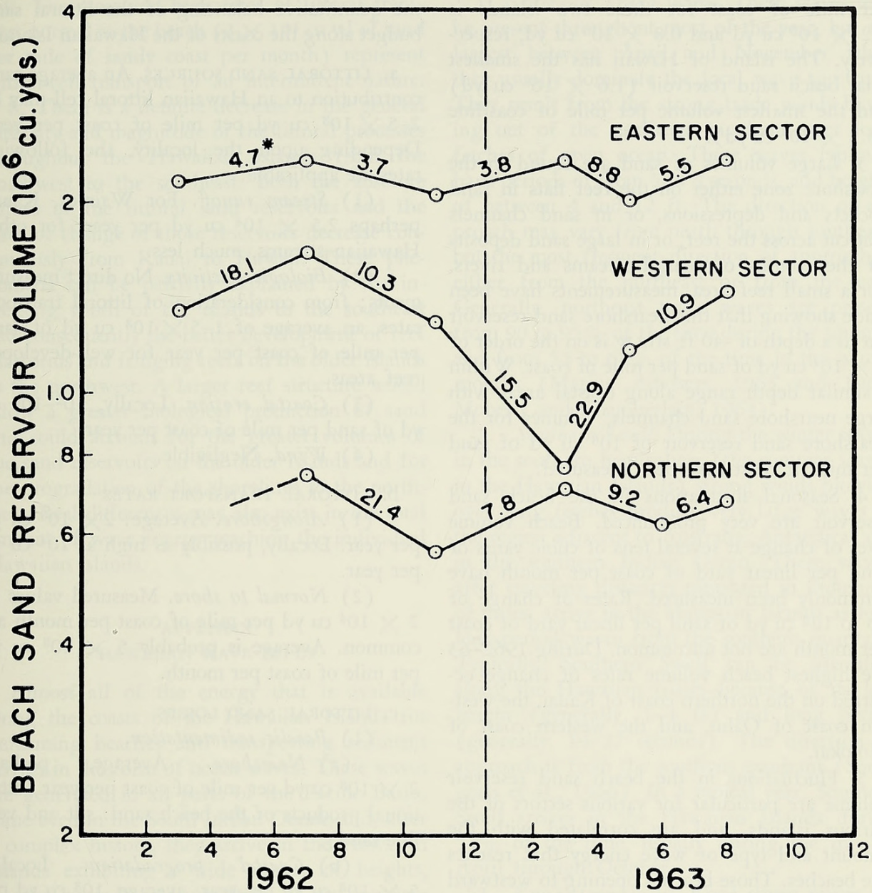
FIG. 6. Seasonal fluctuations in beach sand reservoirs, selected beaches, northern, western, and eastern sectors, Oahu. (*Rates of accretion and erosion in cubic yards/yard of beach/month.)
