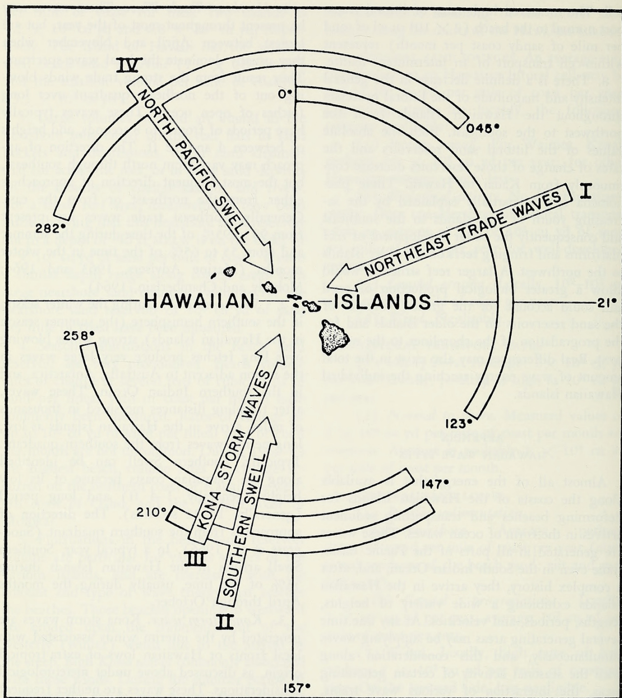
FIG. A-1. Hawaiian waves.
