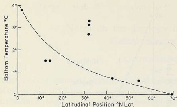
FIG. 2. Relationship between bottom temperatures ( ^{\circ}\text{C} ) and the latitudinal position of species of Galathealinum .
