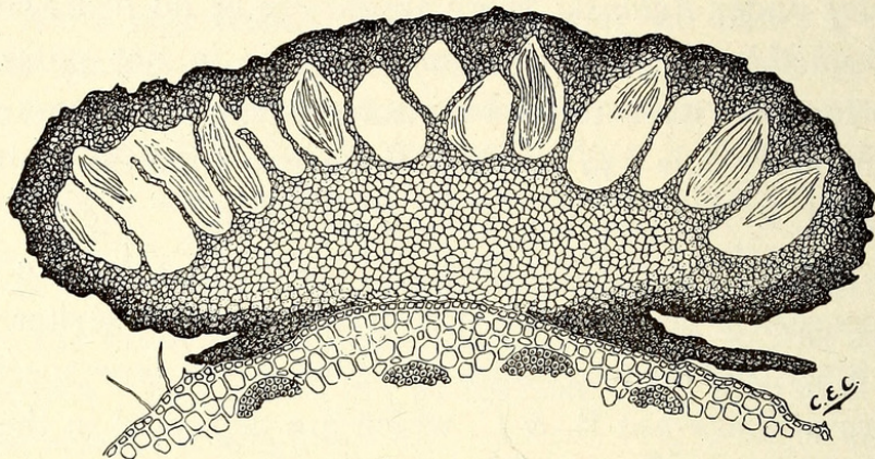
FIG. 1. Dothichloe subnodosa sp. nov. Cross section of a stroma showing the sharp definition between the host and fungous tissue. (Outlined with a camera lucida; \times 50 ).
