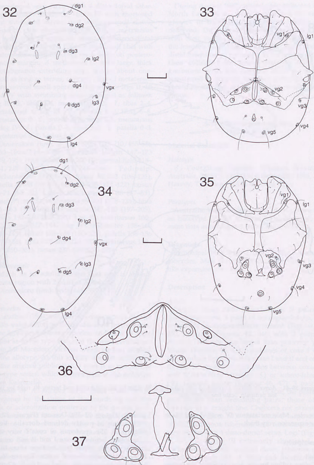
Figures 32-37 Acercella falcipes Lundblad: 32, dorsal aspect, ♂; 33, ventral aspect, ♂; 34, dorsal aspect, ♀; 35, ventral aspect, ♀; 36, genital field, ♂; 37, genital field, ♀. Scale lines = 100 µm.
