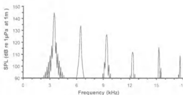
FIG. 3. Spectrum of BASA Technical Services 'whale' alarm.
