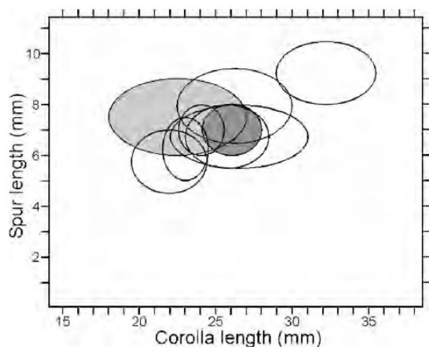
Figure 5: Data from Figure 4 repeated. Also shown are the inner character ellipses for the Castle Crag data (dark grey) and Casper's values for Pinguicula macroceras s. lat. (light grey). Notice that both are reasonably coincident with the range of Pinguicula macroceras in Del Norte County.
