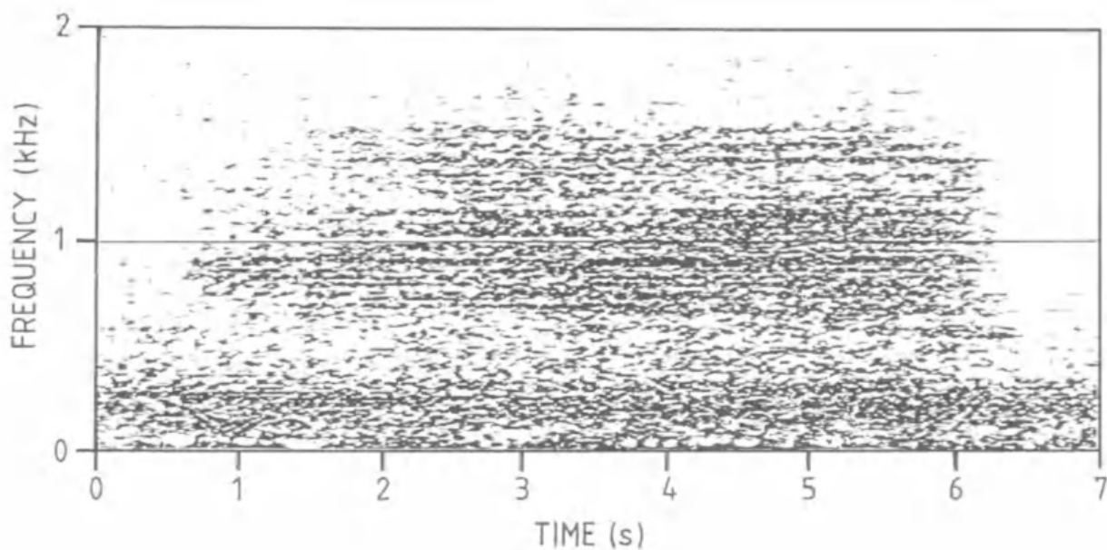
FIG. 6. Sonagram of a broad band with spectral lines sound type "chain-saw growl".
