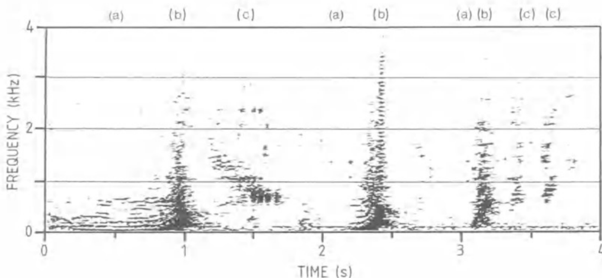
FIG. 8. Sonogram of a complex sound type - "whoomp", including (a) harmonic, (b) impulse, and (c) pulsating ending.
