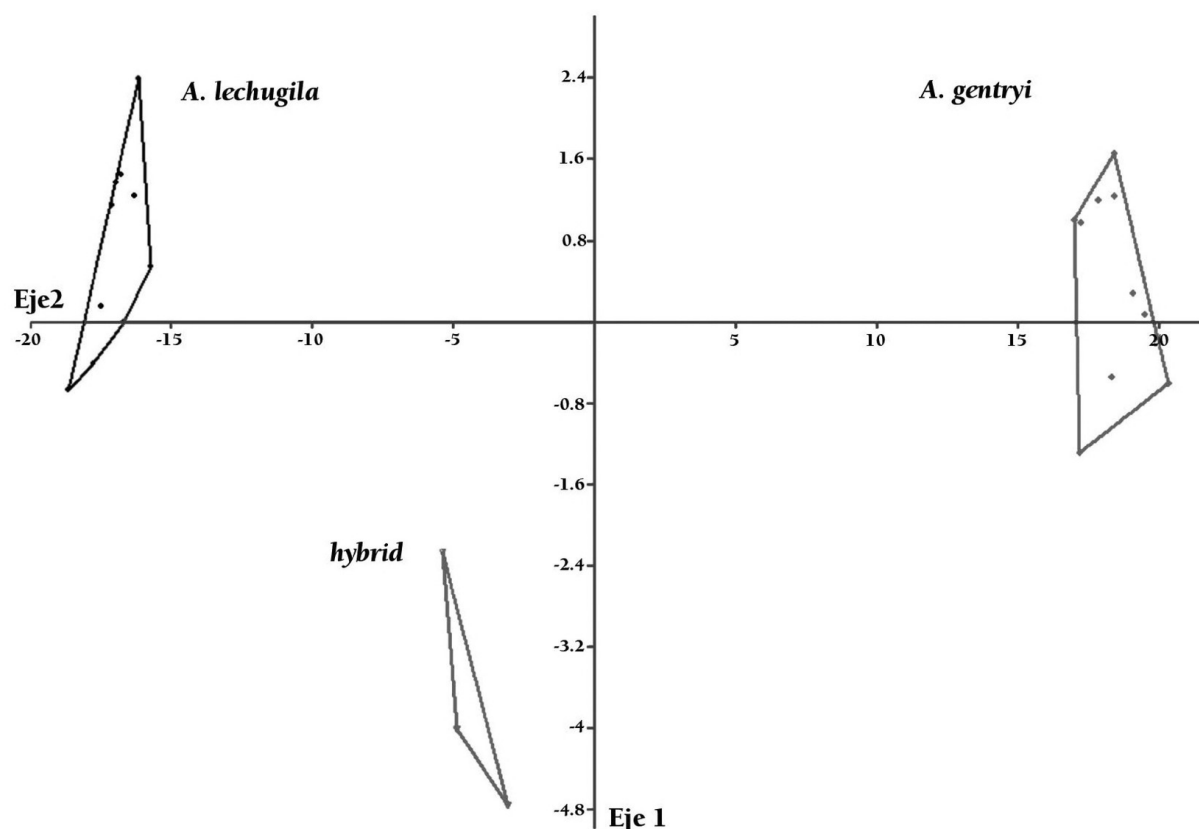
FIG. 1. Plot that shows the results of the use of the Discriminant analysis applied to the five morphometric ratios listed in the Table 2.
