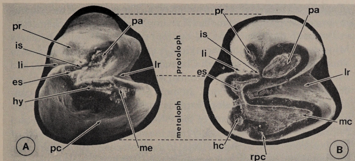
FIG. 1.—Upper premolars of Pliosaccomys higginsensis , Higgins local fauna, early Hemphillian land mammal age, mid-Miocene; A, enamel cap almost unworn; B, enamel cap lightly worn. Abbreviations: pr, protocone; pa, paracone; lr, labial re-entrant; me, metacone; pc, posterior cingulum; hy, hypocone; rpc, remnant of posterior cingulum; es, entostyle; li, lingual re-entrant; is, isthmus.
