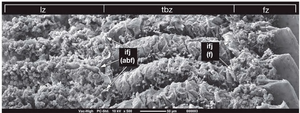
Figure 4. Scanning electron micrograph of the ctenidium of Conchocele bisecta showing details of the frontal, tubular and laminar zones. fz frontal zone; ifj (abf) inter filamentar junctions, abfrontal; ifj (f) inter filamentar junctions, frontal; lz laminar zone; tbz tubular zone.
