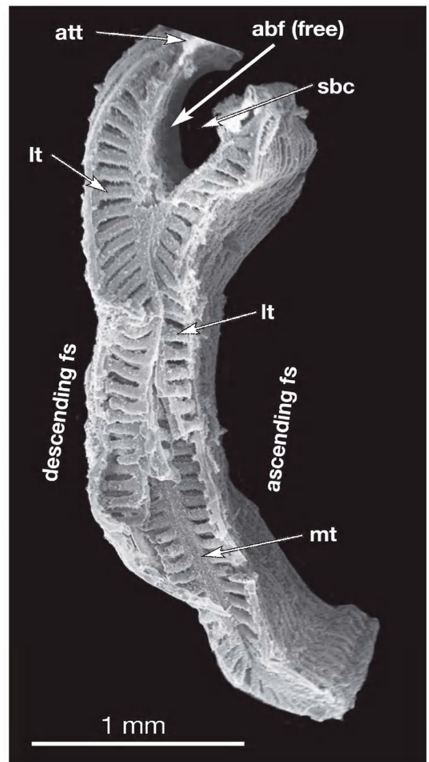
Figure 5. Scanning electron micrograph of the ctenidium of Ochetoctena tomasi , lateral view of a filament. abf (free) free abfrontal surface; att attachment point; fs frontal surface; lt lateral tubule; mt median tubule; sbc supra branchial chamber.
