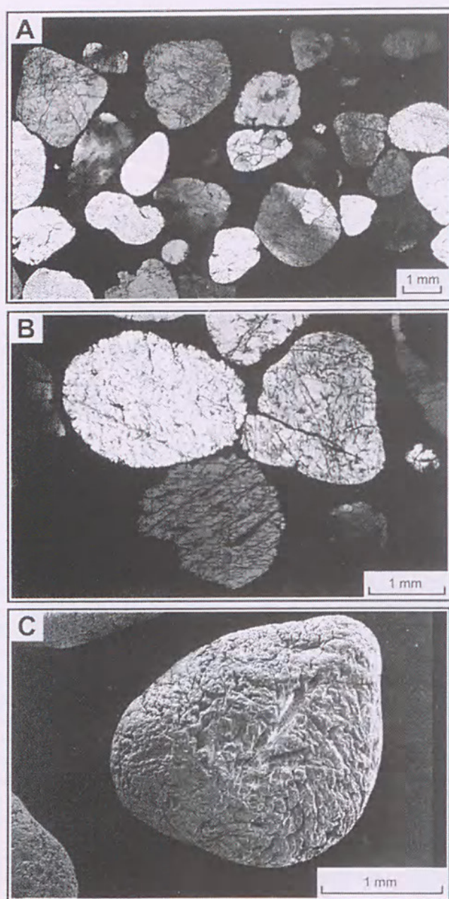
Figure 9. A–C: Rounded, very coarse sand-sized quartz grains in the Westonia Formation. The rounded quartz grains were probably ultimately sourced from an ancient texturally mature (?fluvial) sediment. A,B = sample EY61/1 optical photomicrographs cross-polarized light. C = sample EY61/1 scanning electron photomicrograph.
