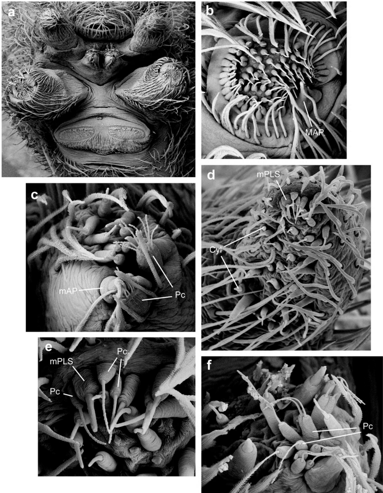
Figure 3. a–e, spinnerets, Therlinya kiah (KS3659, ♀): a, spinning field; b, ALS; c, PMS; d, PLS; e, detail of PLS apex with modified PLS spigot. f, PMS, Baiami brockmani (♀), arrows to a single and a double Pc spigot base. Spigots: MAP, major ampullate; mAP, minor ampullate; Cyl, cylindrical; mPLS, modified posterior lateral spinneret; Pc, paracribellar
