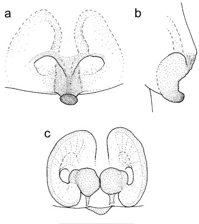
Figure 16. Therlinya nasuta . a–c, epigynum (holotype): a, ventral, b, lateral; c, dorsal—internal genitalia (S42264). Scale line 0.5 mm.
