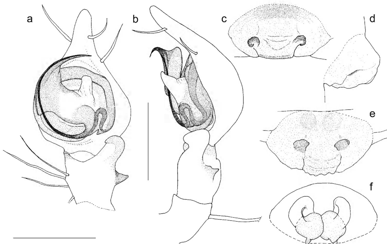
Figure 8. Therlinya horsemannae . a,b, male palp (holotype): a, ventral; b, retrolateral. c–f, epigynum (KS58197): c, ventral; d, lateral; e, posterior; f, dorsal—internal genitalia. Scale lines 0.5 mm: vertical, a,b; horizontal, c–f.
