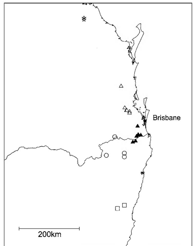
Figure 12. Distribution of Therlinya species: northern New South Wales and southeast Queensland. ▲ T. wiangaree , △ T. vexillum , ☆ T. horsemannae , ○ T. ballata , □ T. bellinger .
