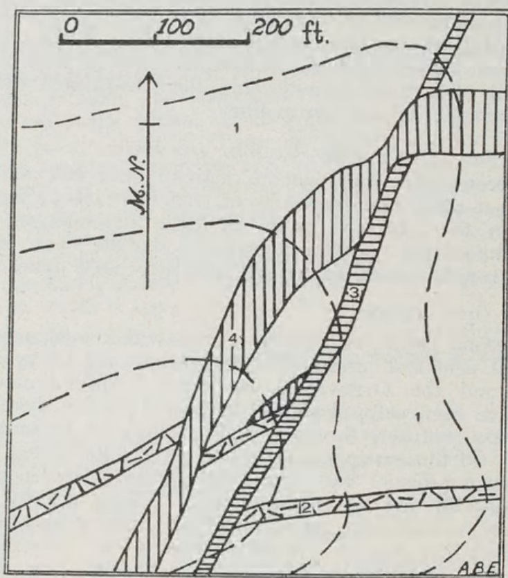
Fig. 2. Dyke Sequence in Allotment 81, Parish of Cudgewa. 1. Grey Corryong Granite. 2. White Granite Dyke. 3. Granophyric Quartz-Porphyry Dyke. 4. Quartz-diorite Dyke.
