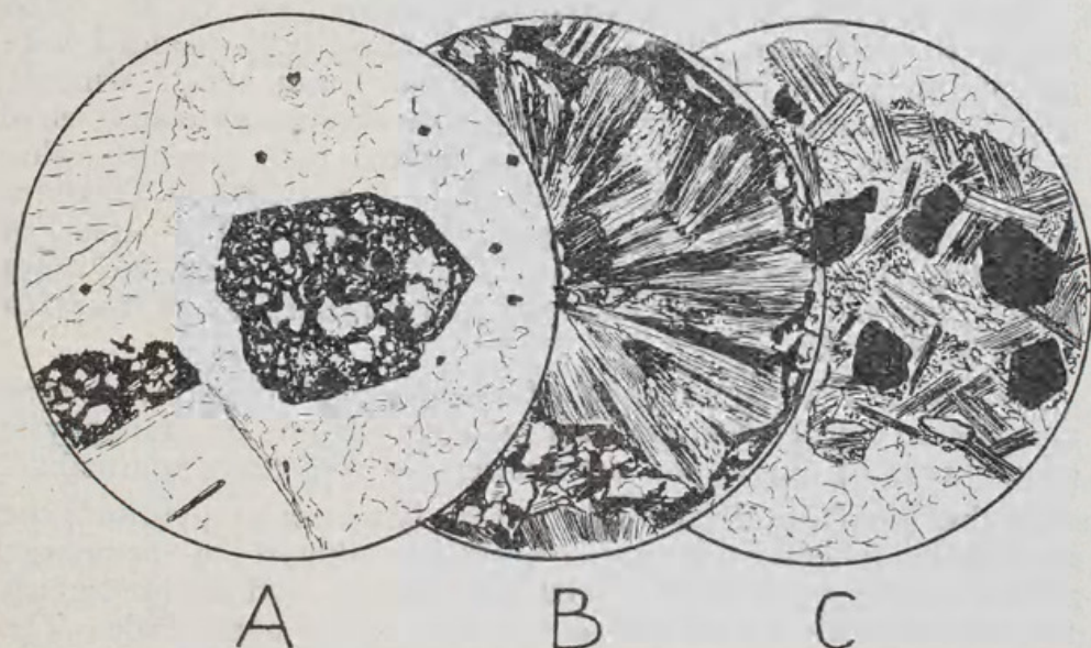
Fig. 4. A. Micro-"quartz-tourmaline nodule" in quartz-porphyry. \times 200 .
