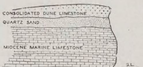
FIG. 3.—Sea cliff on headland forming east side of Stanhope Bay. The cliff is approximately 120 feet high, consisting of about 80 feet of Miocene marine limestone, about 20 feet of fine quartz sand, and about 20 feet of hard dune rock.
