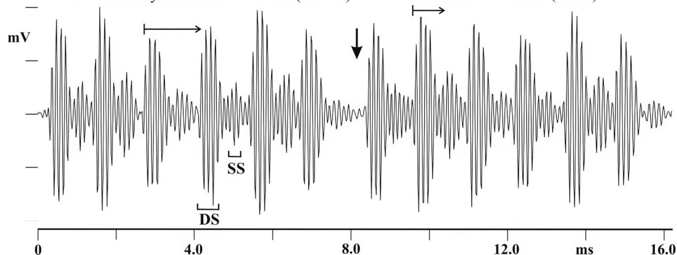
Figure 5. Arenopsaltria nubivena , waveform plots of calling songs from 5.6 km west of Windorah, southwest Queensland; (A) general view showing the relatively uniform, continuous buzzing song, but showing two short breaks (marked by hollow arrows); (B) time expanded segment of calling song showing the repeated macrosyllables, each with six dominant syllables, the arrows defining the limits of the individual macrosyllables; (C) higher resolution waveform plot of two macrosyllables, the filled arrow marking the boundary between the macrosyllables. The six dominant syllables (DS) each comprise 5 to 7 high amplitude carrier wave pulses. The time intervals between the dominant and secondary syllables (SS) comprise lower amplitude background pulses, variably frequency modulated; the horizontal arrows define the syllable repetition rates (RR) and the intra-syllable durations between the dominant and secondary syllables. Field recordings, filtered to 1 kHz.
