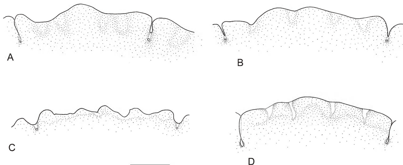
Figure 3. Lappets, oral view. (A) Cassiopea ndrosia , Lake Illawarra, bd 80 mm, AM G.18075. (B) Cassiopea ndrosia , bd 100 mm, Hayman Island, AM G.13568. (C) Cassiopea cf. maremetens , bd 90 mm, Wallis Lake, AM G.18156. (D) Cassiopea maremetens , paratype, bd 110 mm, Moreton Bay, QM G6645. Scale = 5.0 mm.
