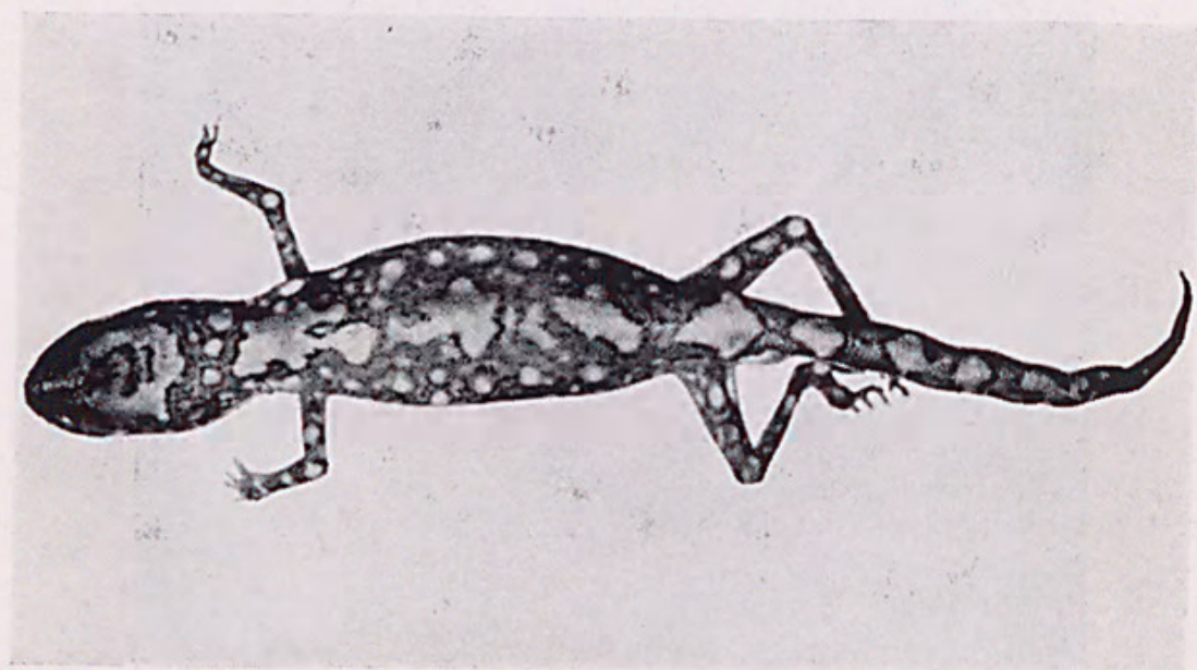
Fig. 2.—A dorsal view of the holotype of Diplodactylus squarrosus .
