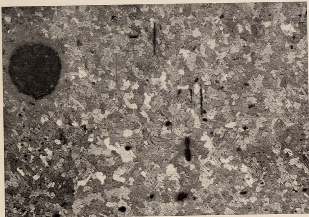
THE STRTCTURE OF METEORITES A section of Williamette showing its granular structure; the Widmanstätten lines are very faint
