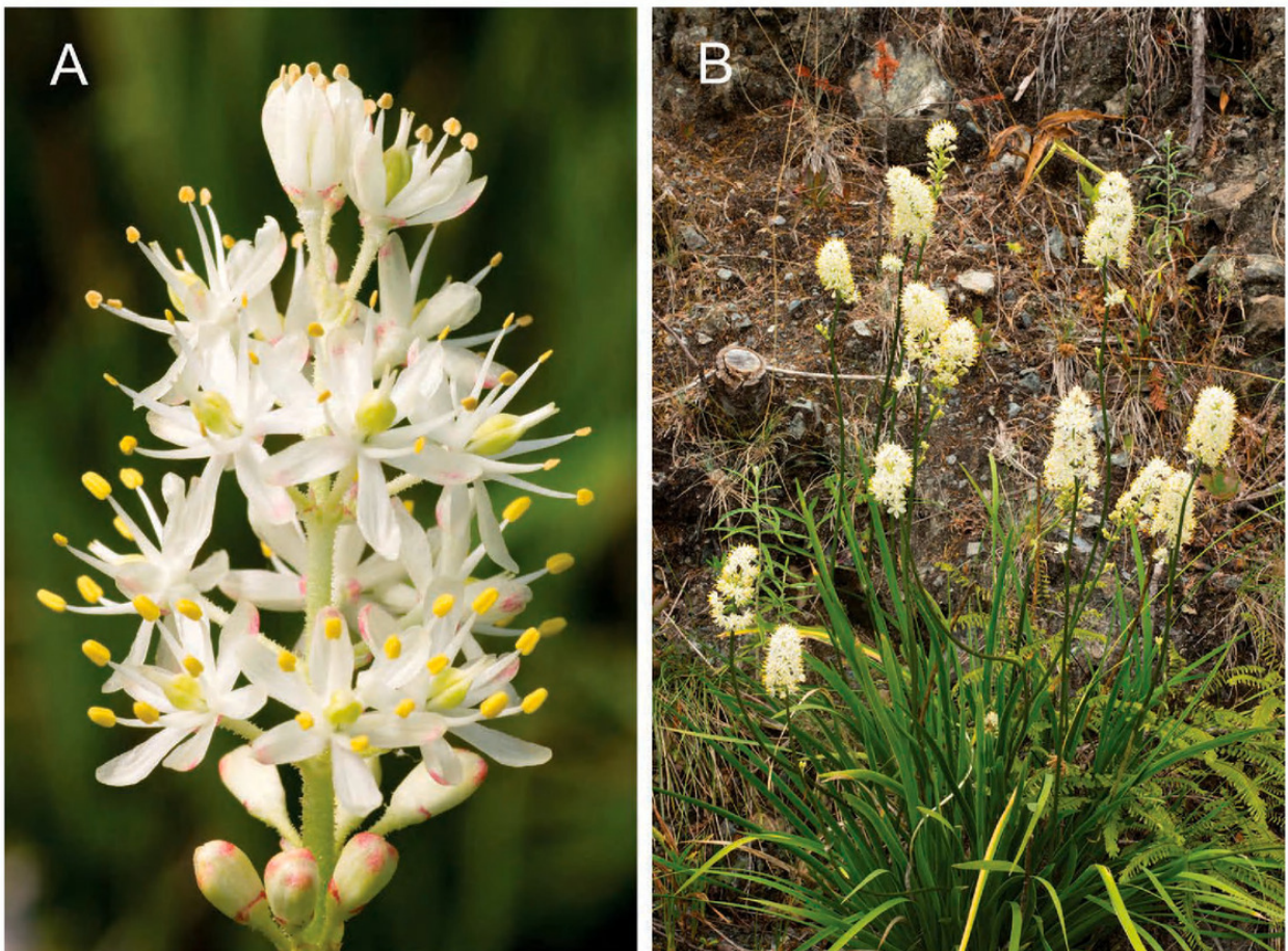
Figure 1: (A): Triantha occidentalis subsp. occidentalis in Plumas County (California). Can you see the small, glandular hairs on the inflorescence, and also can you see the groupings of flowers in threes? (B): Triantha occidentalis subsp. occidentalis in Del Norte County (California). The inflorescences of these plants are so large, they start to look like Toxicoscordion (= Zigadenus ), in the closely related family Melanthiaceae.
