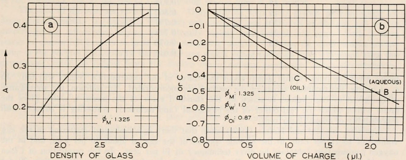
FIGURE 1. Graphs for calculating the values of the constants A , B and C in the formula for V , the total gas space of the charged diver at equilibrium pressure.
