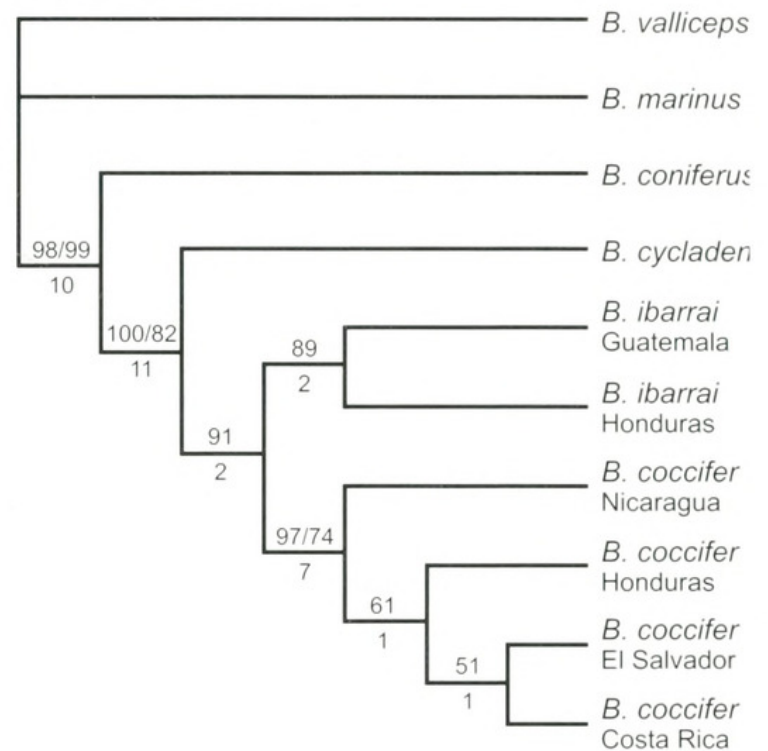
Fig. 14. Phylogenetic relationships among samples used in molecular analyses; see Table 4 for specimen information. Topology is shown from the maximum-parsimony exhaustive search. Bootstrap values greater than 50% (MP/ML) are shown for each analysis above branches and decay indices are shown below.
