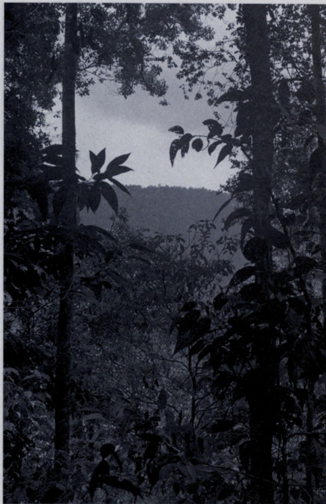
FIG. 4. Photograph of habitat at 1100 m (Site 2) in April 1992.
