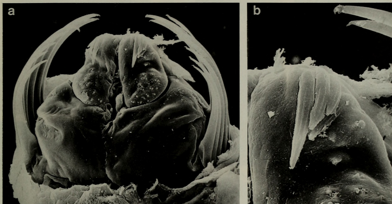
Fig. 2. SEM photographs of Spadella japonica , new species: a, Ventral part of head ( \times 180 ); b, Details of teeth ( \times 500 ).
