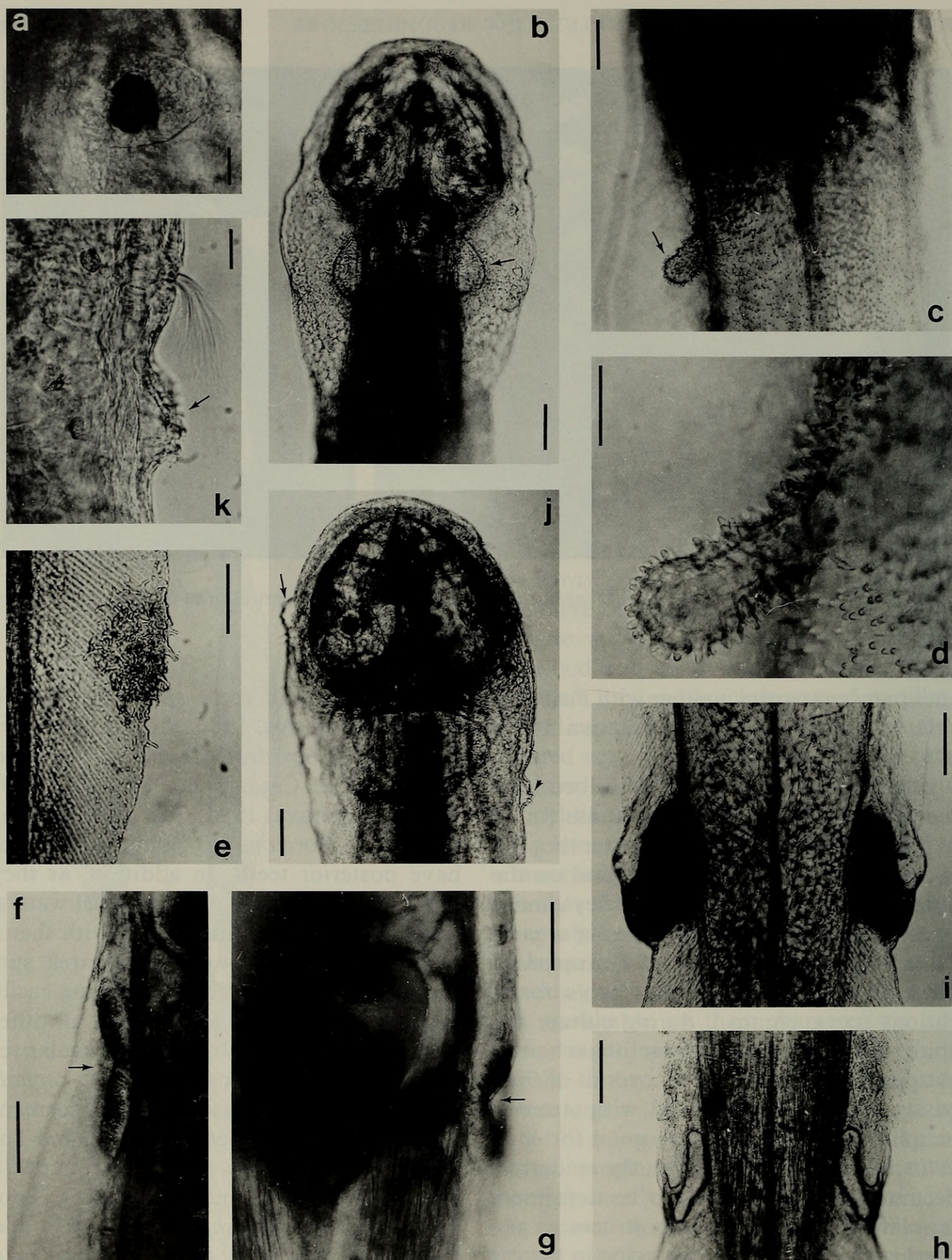
Fig. 3. Spadella japonica , new species: a, Right eye; b, Anterior part of body in dorsal view showing the corona ciliata (arrow); c, Anterior part of the tail of an original specimen in ventral view, showing a curious "papillated organ" (arrow) and adhesive papillae; d, Enlargement of the "papillated organ" area; e, Area with tiny papillae on the ventral side of the left lateral fin (other original specimen); f and g, Two aspects of the female genital opening (arrow) in dorsal view; h, Empty seminal vesicles; i, Mature seminal vesicles; j, Head and neck of another original specimen with two "papillated organs" (arrows) in dorsal view; k, Enlargement of the organ on neck (arrow), just under a sensory spot. Scale bars: 0.1 mm (b, c, e-j), 0.05 mm (d) and 0.02 mm (a, k).
