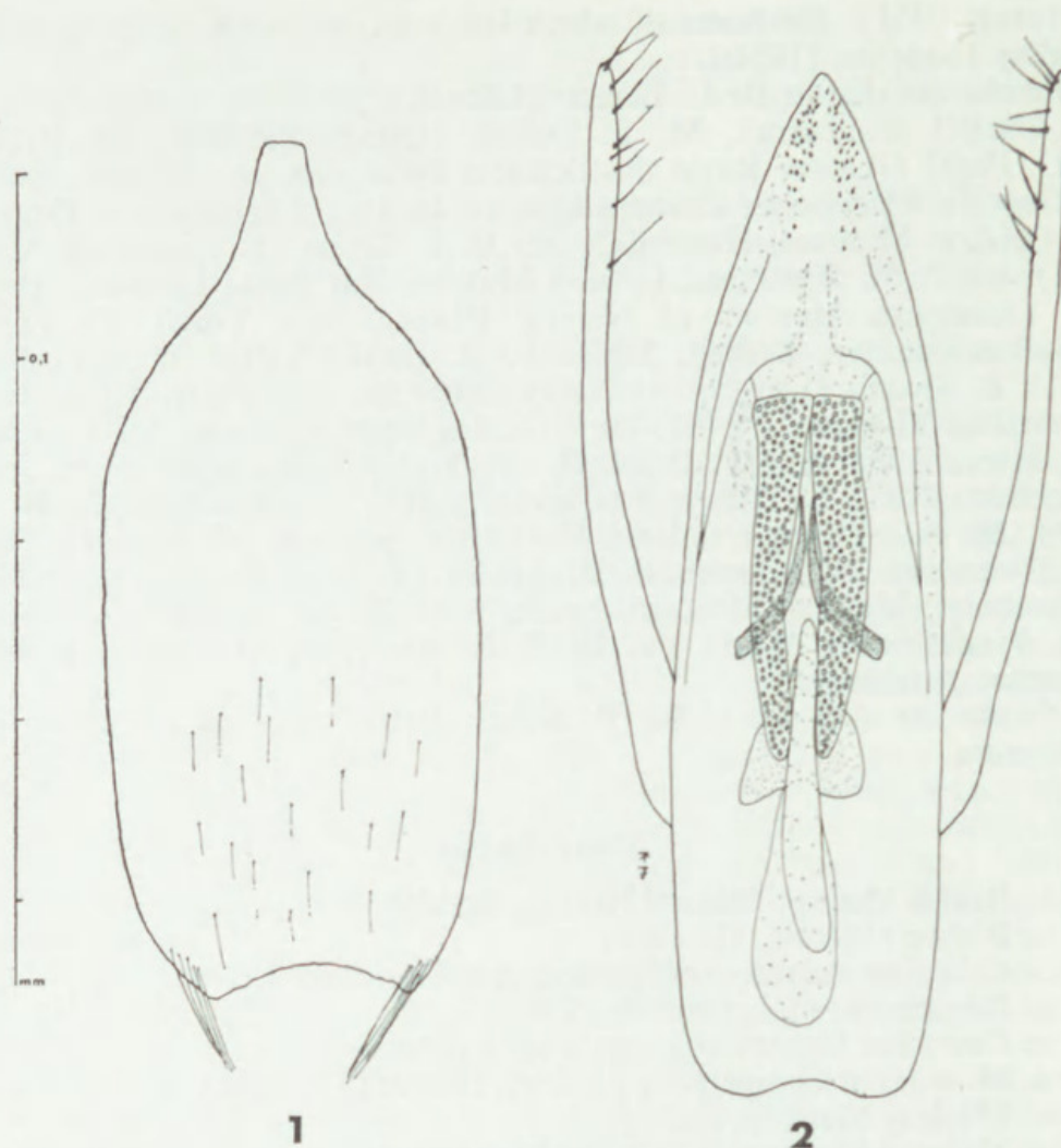
Fig. 1, 2— Stenus cupreipennis Macleay (Qld). 1: 9th sternite of ♂. 2: Ventral aspect of aedeagus.
