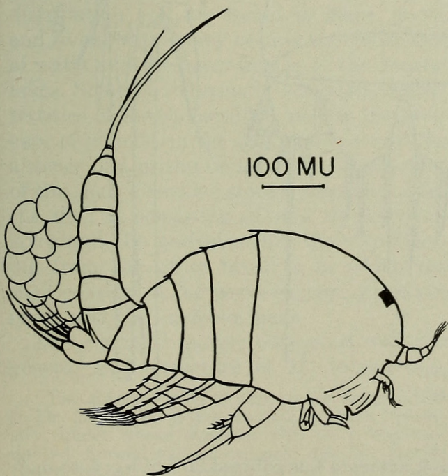
FIG. 1.— Diarthrodes cystoeccus , n. sp., mature female.
