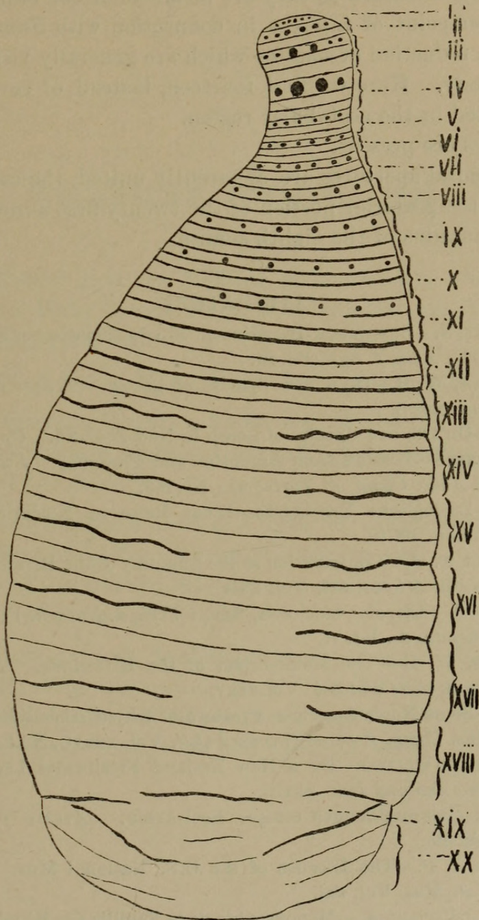
Fig. 13.— Semilageneta Hilli , gen. et sp.n. Diagram showing the metamer arrangement in the annuli.
