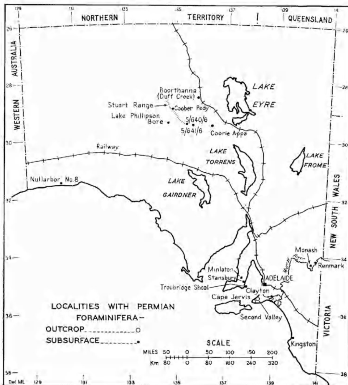
Fig. 1. Map showing localities with Permian foraminifera.
