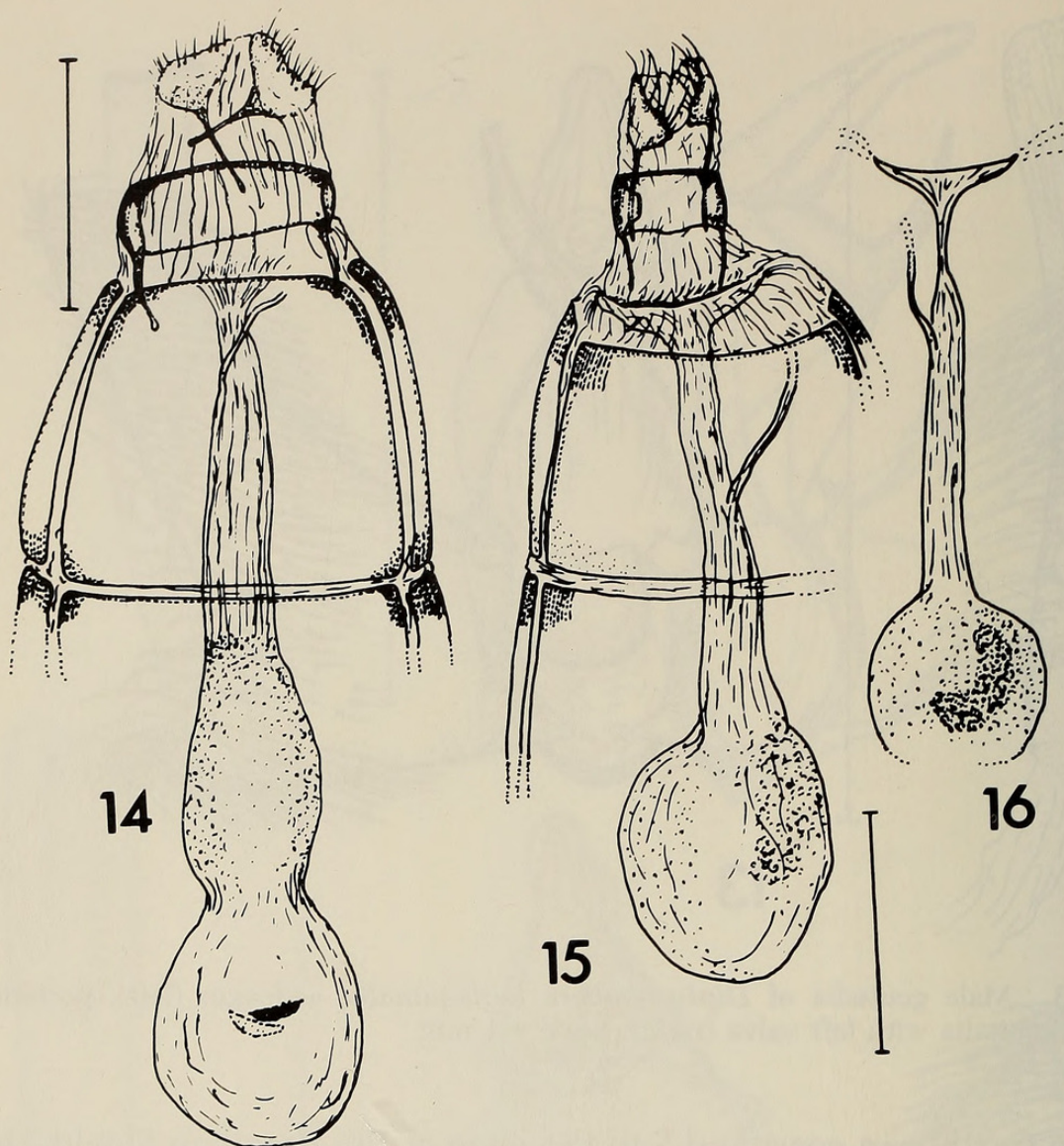
FIGS. 14-16. Female genitalia of Diptychophora , ventral aspect. 14, D. kuhlweini ; 15, D. subazanalys paratype; 16, D. subazanalys variation in form of signum. Scale = 1 mm.
