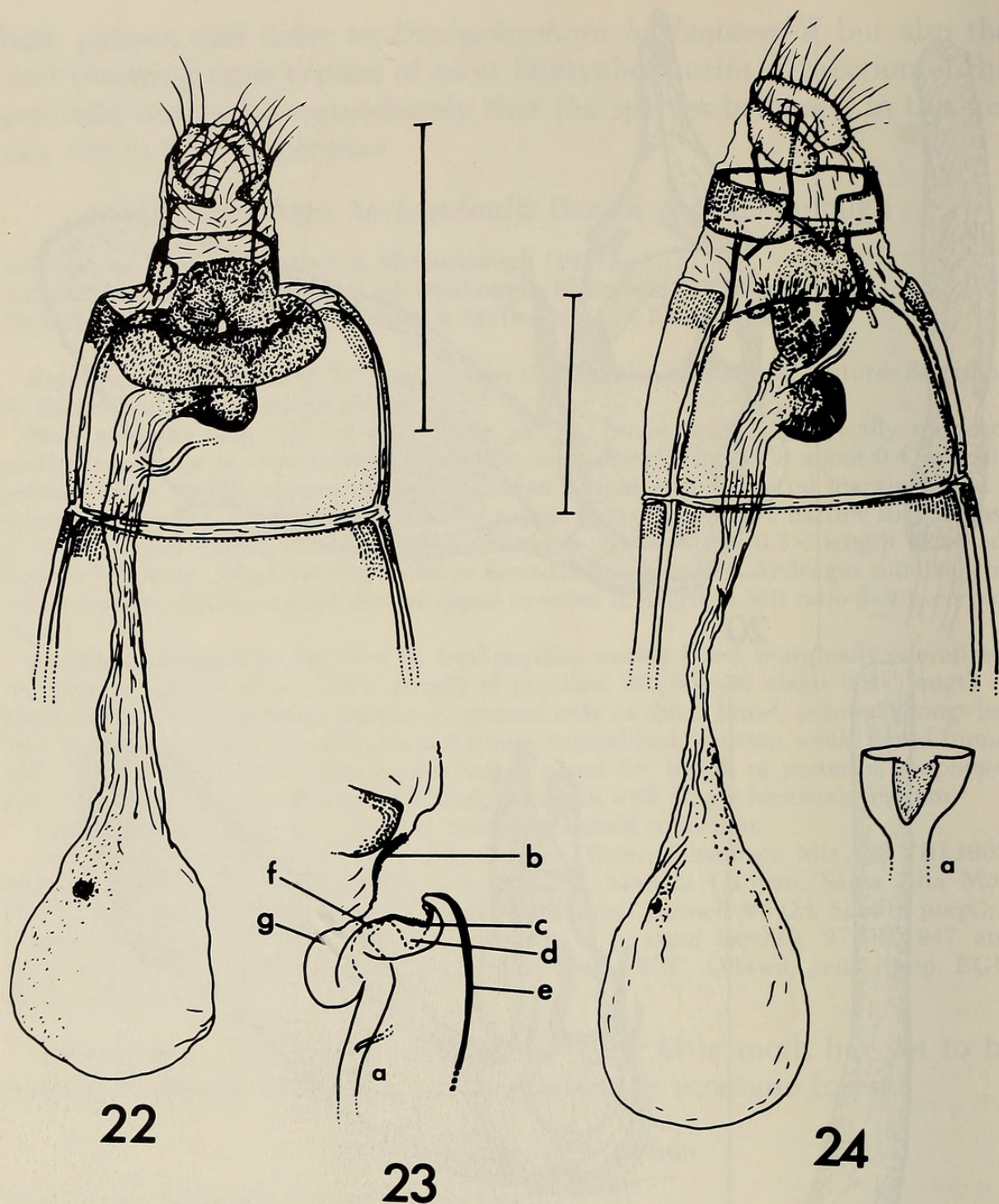
FIGS. 22-24. Female genitalia of Steneromene . 22 , S. azanalis holotype, ventral aspect; 23 , S. azanalis , diagram of antrum in lateral aspect, a, ductus bursae; b, lamella postvaginalis; c, lamella antevaginalis; d, antral "pocket"; e, 7th sternum; f, antrum; g, subantral expansion; 24 , S. nymphocharis lectotype, ventral aspect, a, diagram of antrum, ventral aspect.
