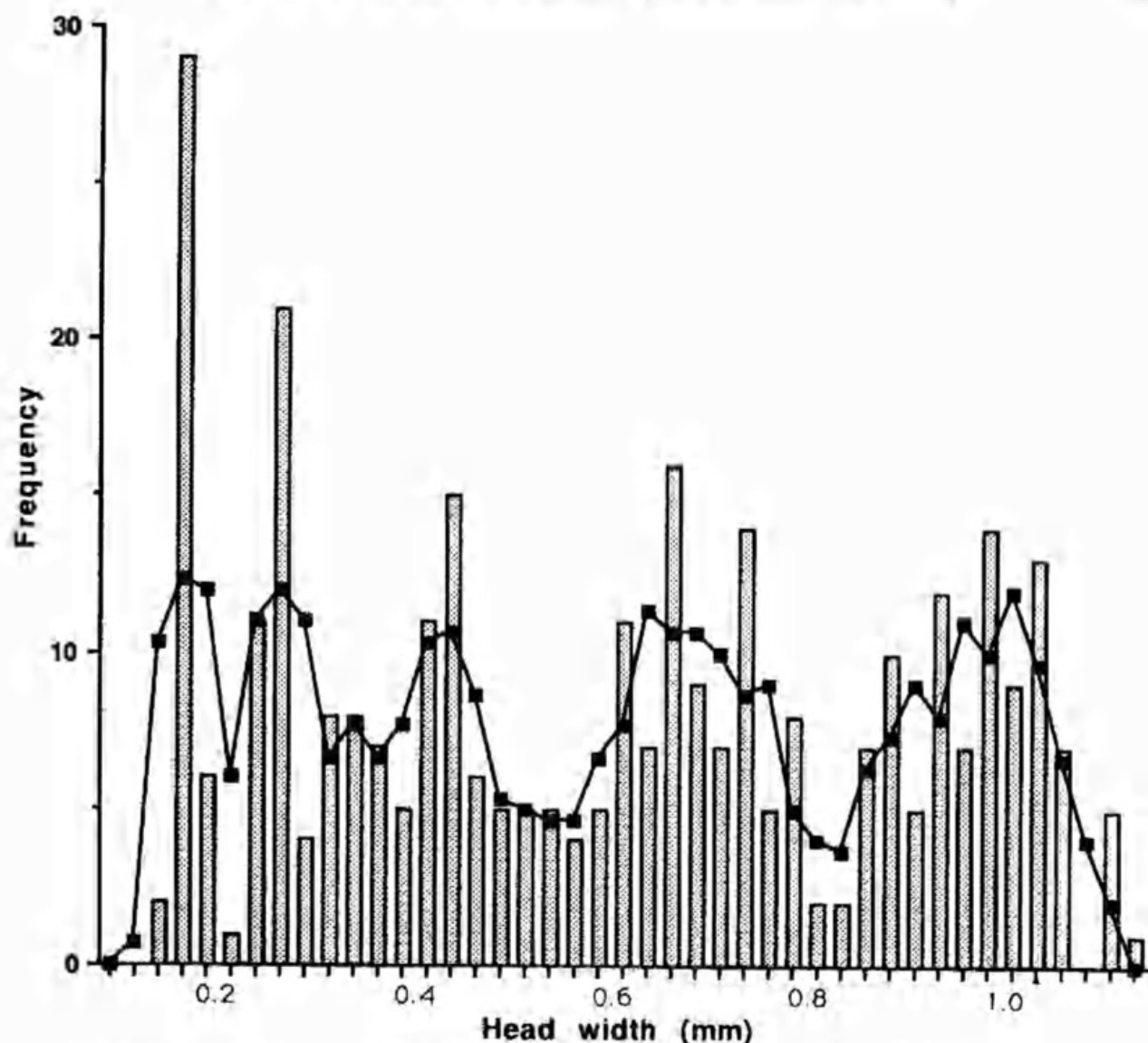
Fig. 3. Head capsule widths of larvae of Etella behrii collected randomly from the field at 'Brecon' (Keith) ( n = 329 ), expressed as a frequency distribution (histogram) and three-point moving averages (■).
