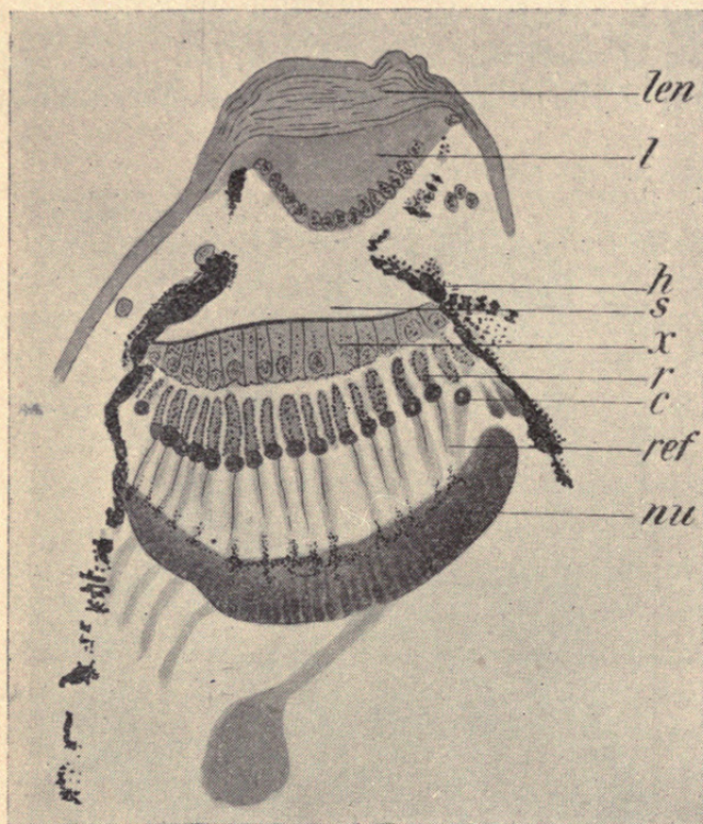
FIG. 5.—Section of left eye of the posterior and ventral pair, transverse to axis of body. Lens crinkled and hypodermis ruptured (abbreviations as in Fig. 4). \times 300 .
